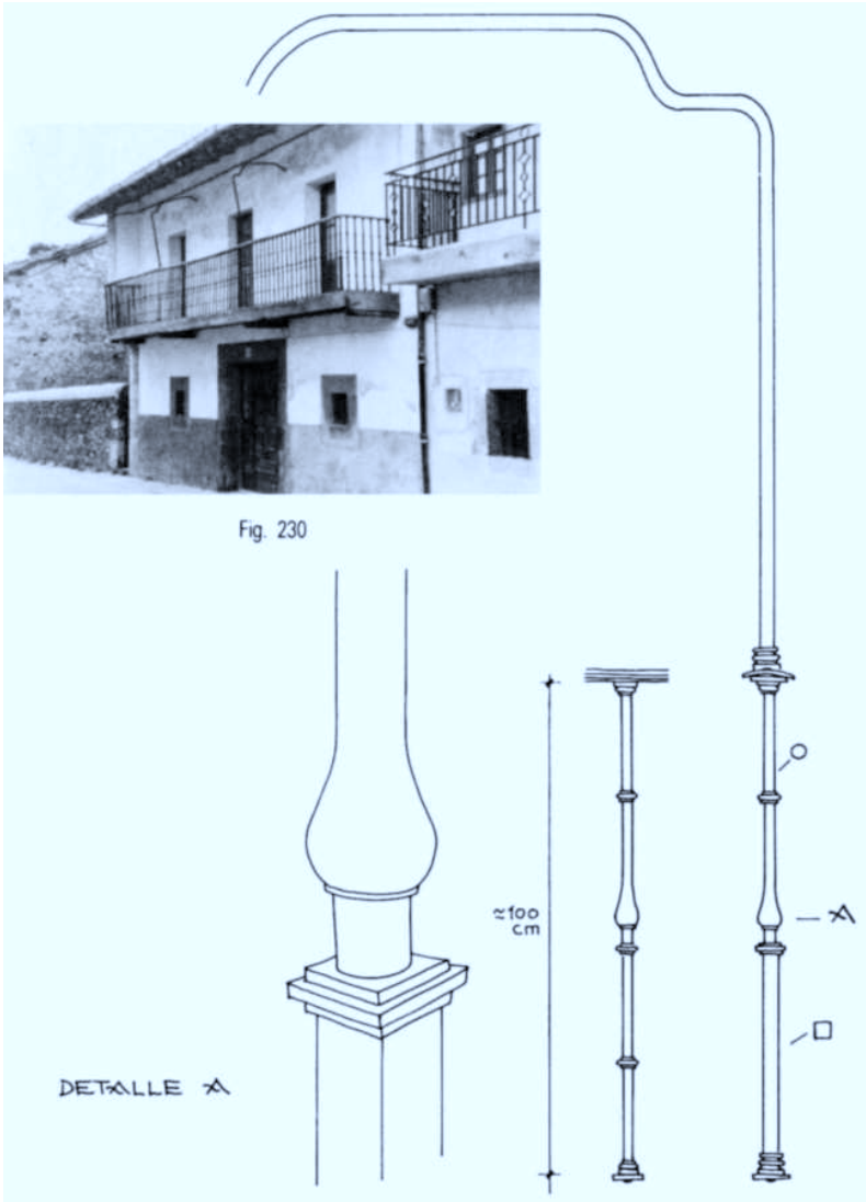
BARROTES DEL BALCON
