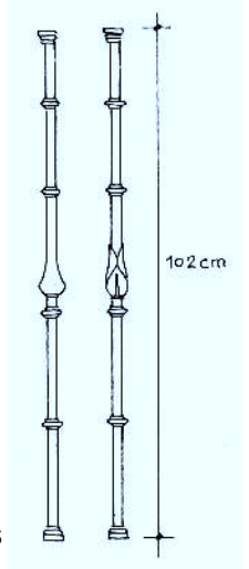
BARROTES DEL BALCON
