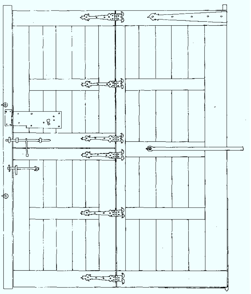
PUERTA PRINCIPAL VISTA INTERIOR
