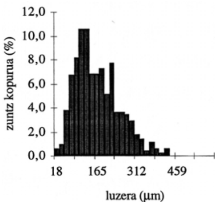
(a) GPES 30: L_n = 175 \mu\text{m}
