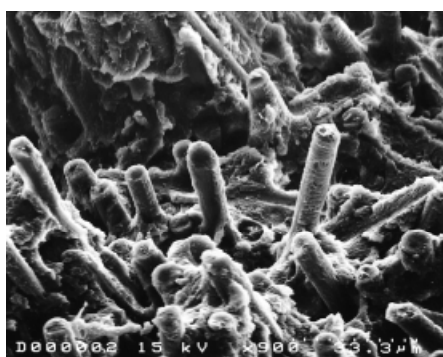
(c) PEEK/CF
