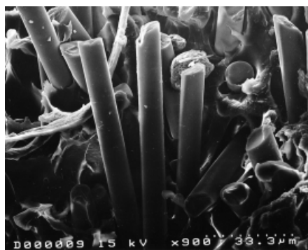
(a) PEEK/GF
