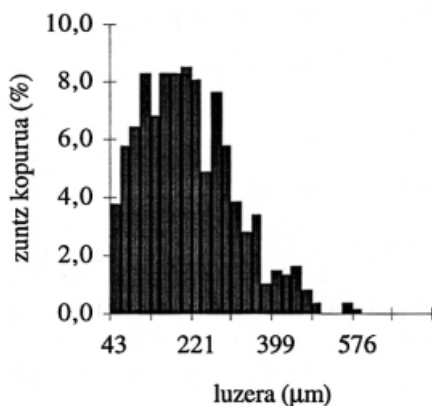
(a) GPEEK 30: L_n = 176 \mu\text{m}
